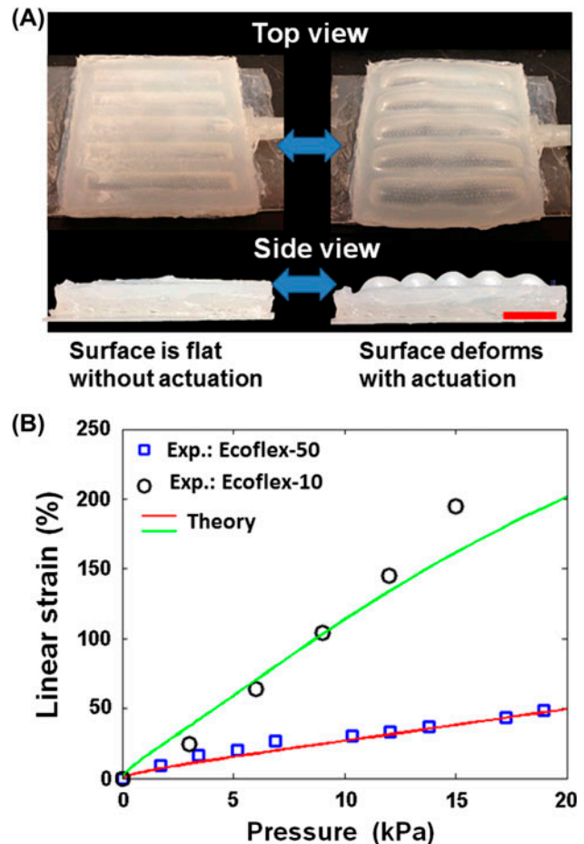
Figure 1. Optical photographs of a pneumatic network (Ecoflex-10) that shows the surface to be flat without actuation and undergoes deformation when pneumatic pressure is applied (A). The scale bar (red) represents 12 mm. Relationship of applied internal pressure by pneumatic actuation on strain generated on the surface of Ecoflex-10 and Ecoflex-50 (B); the experimental data match with the theoretical predicted strain using a 2D plane-strain model.
